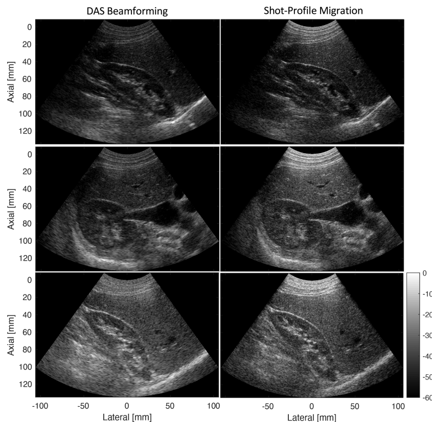
Fig. 4. Comparison of shot-profile migration to DAS beamforming based on virtual-source synthetic aperture for a focused transmit sequence on a Siemens 5C1 probe.
